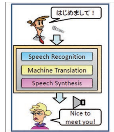
Fig. 1 Speech-to-speech translation
