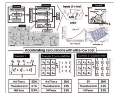
Fig. 2 Analog Accelerators
