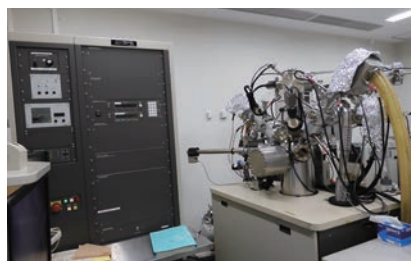
Secondary Ion Mass Spectrometer (SIMS)
