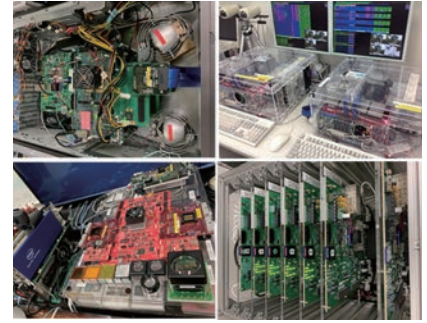
IoT/server acceleration by FPGAs (Computing Architecture Lab)
