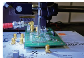
Fig. 3 Evaluation board for physical security evaluation including post-quantum cryptography.
