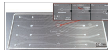
Fig. 3 High-speed laser manipulation in microfluidic chips.
