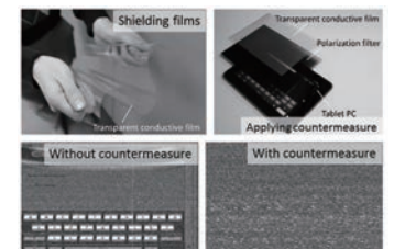
Fig. 2 Development of countermeasures to prevent EM display stealing from tablet PCs
